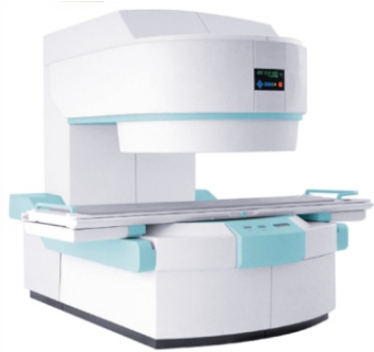
MK-OPERO.4 Permanent-magnet Magnetic Resonance Imaging System Power Output:15KW Inverter Frequency:40kHz
