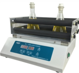
MK-MS1 Intelligent Shaker Working Size: 420x290mm Speed Range: Start up-300rpm Time: 0~99h 59min
