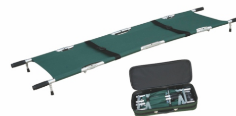
MK03-315 Aluminum Alloy Fold Stretcher Product Size:214x55x12cm Folded Size:58x21x14cm
