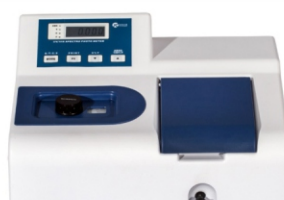
MK-W754 Speetrophotometer Optical system: Czerny-turner CT grating monochromator, 1200/mm Wavelength accuracy: ±3nm
