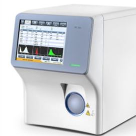
MK-BC-20S 3-Diff Hematology Analyzer CBC+3-DIFF, 19parameters+3histograms Throughput: 40 samples per hour 8.4 inch TFT touch screen Open vial sampling 200,000 results storage with histograms
