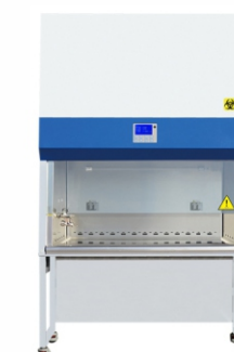
MK-BC86 Class II Biosafety Cabinet External Size: 130x79x231cm Internal Size: 120x60x77cm
